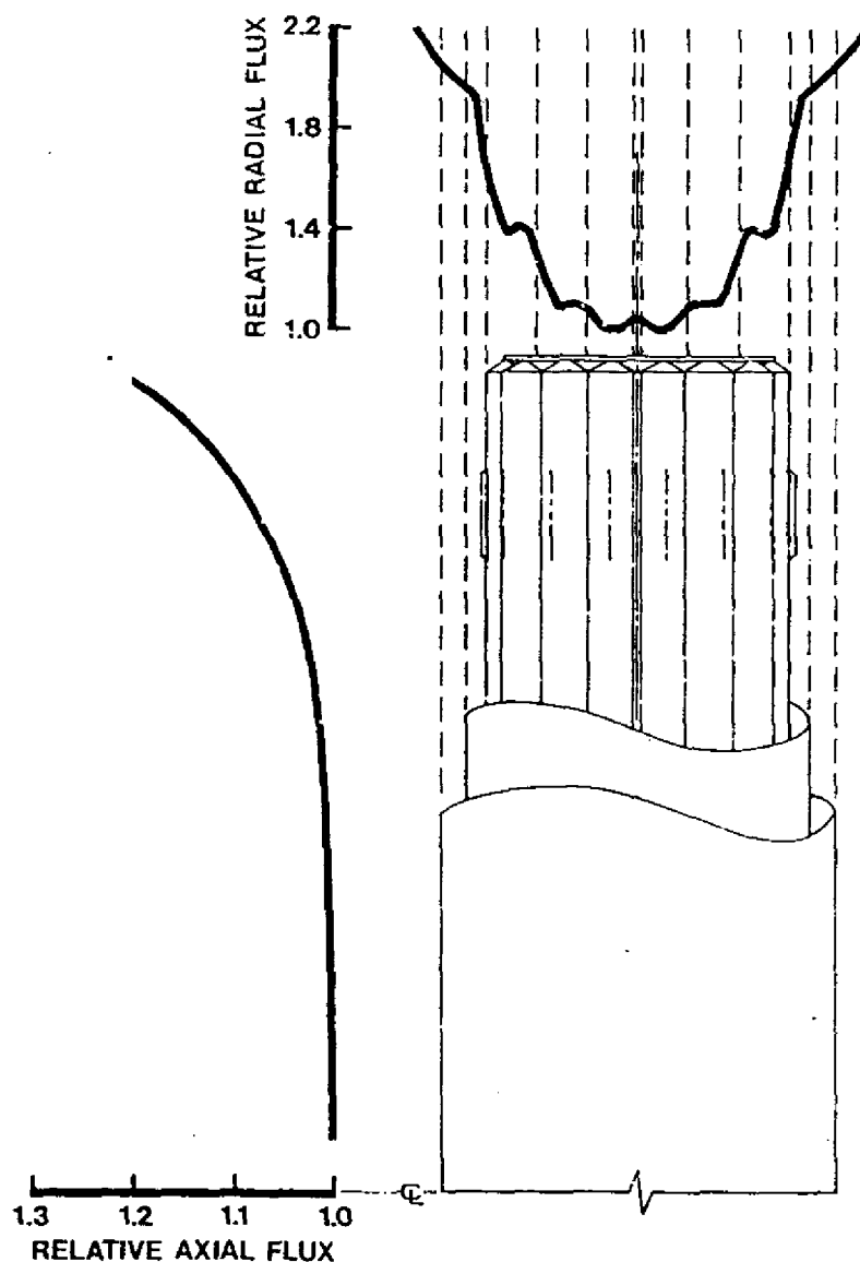
FIGURE 43 Bundle Radial and Axial Flux Distribution
