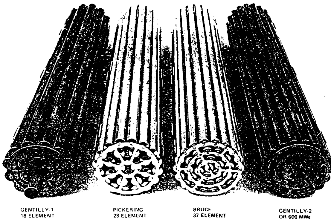
FIGURE 4b Fuels for Canada's Power Reactors, 10 cm Bundles, Pickering, Gentilly-1, Bruce and Gentilly-2
