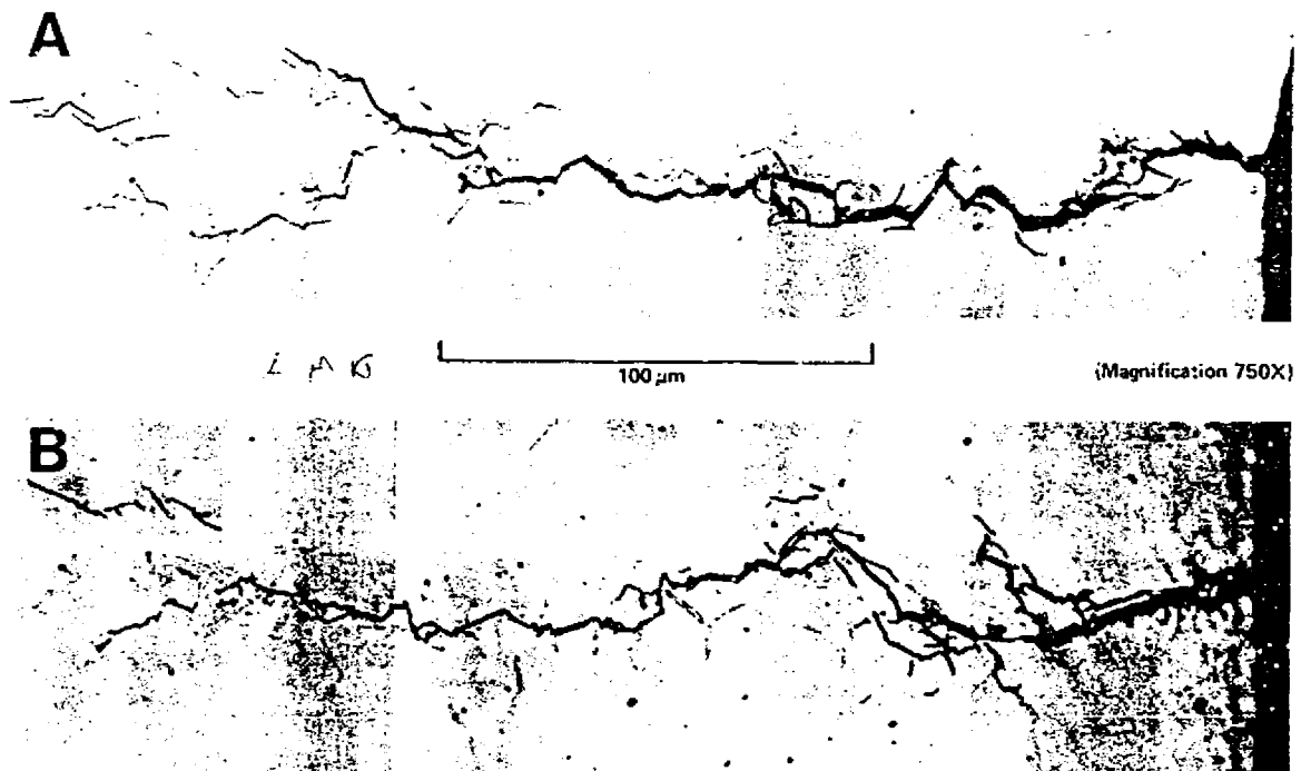
FIGURE 25 Stress Corrosion Cracking
