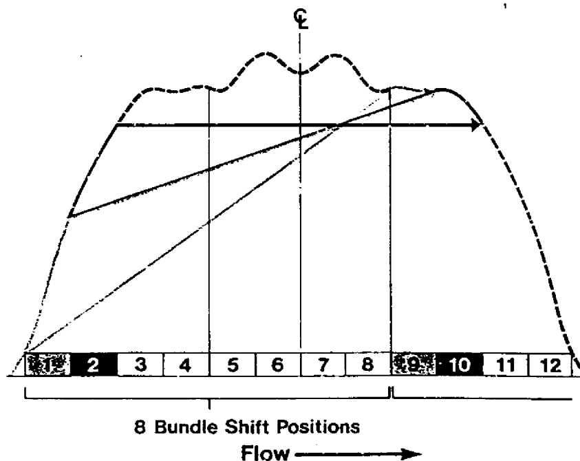
FIGURE 42 Pickering Axial Flux Profile
