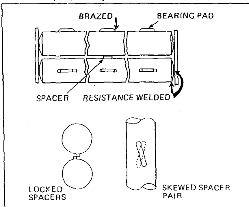
FIGURE 10 Split Spacer Design
