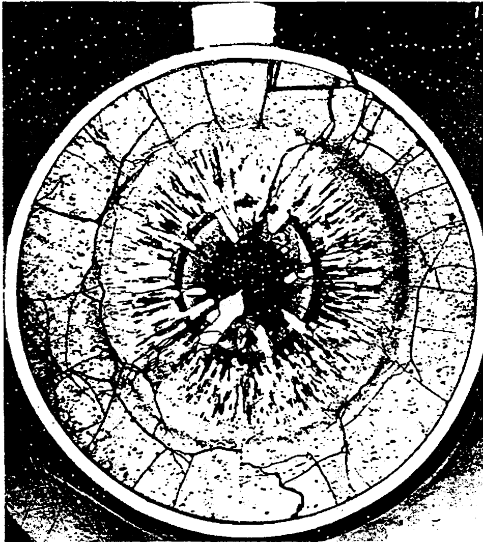
FIGURE 37 Cross Section of Element and Centre Melting in \text{UO}_2
