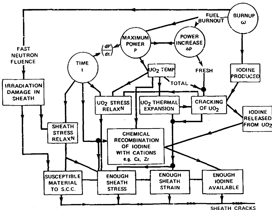
FIGURE 35 Stress Corrosion Cracking Model
