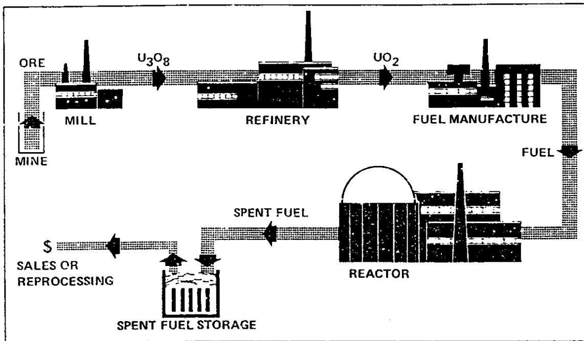
FIGURE 5 Natural Uranium Cycle
