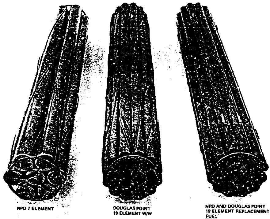
FIGURE 4a Fuels for Canada's Power Reactor, 8 cm Bundles, NPD, Douglas Point
