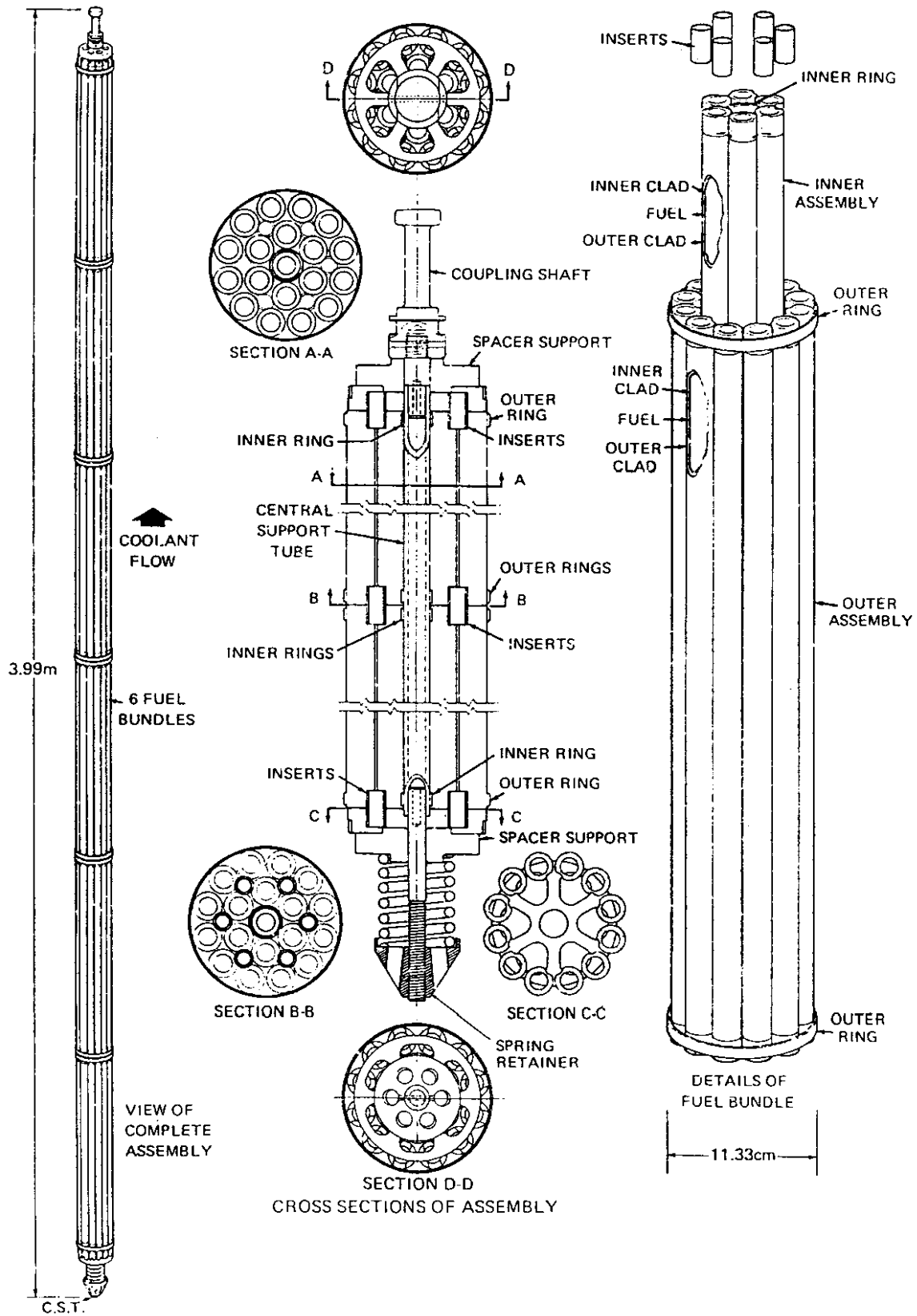
FIGURE 45 Bruce Booster Fuel String Assembly
