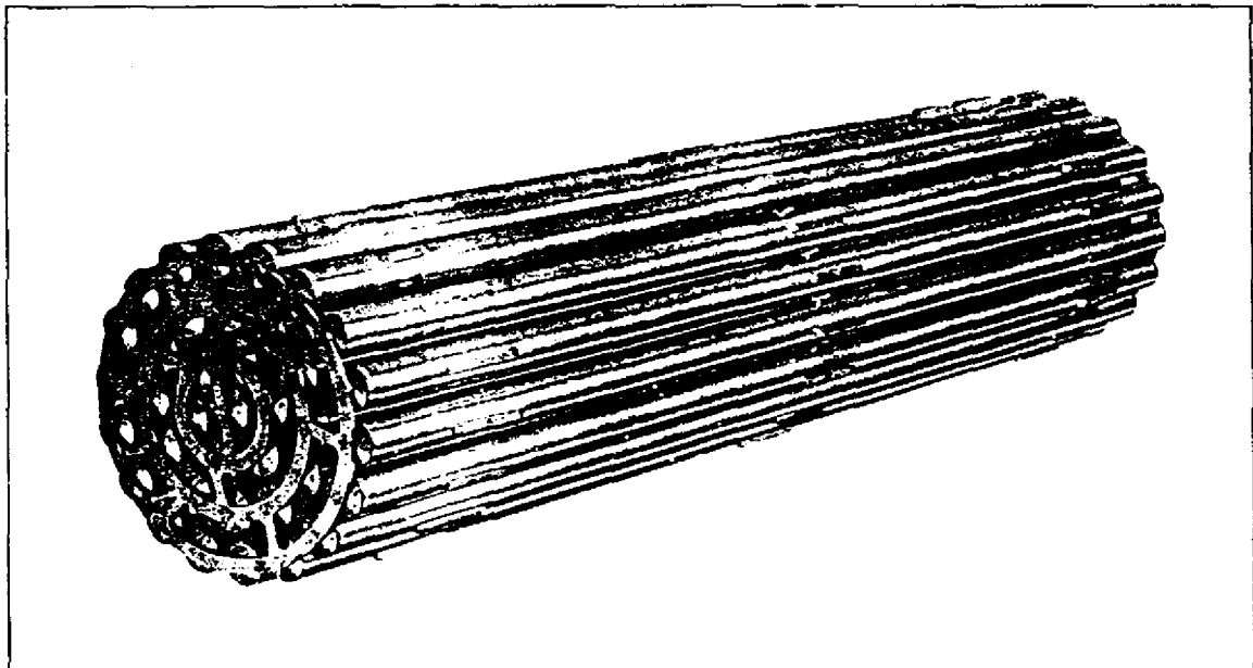
FIGURE 2b 600 MWe Gentilly-2 37-Element Fuel Bundle
