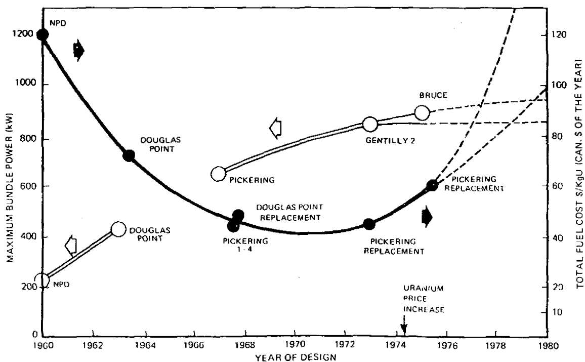
FIGURE 50 Variation of Bundle Power and Fuel Costs showing Evolution with Time
