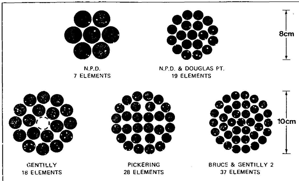
FIGURE 3 Fuel Bundle Cross Sections
