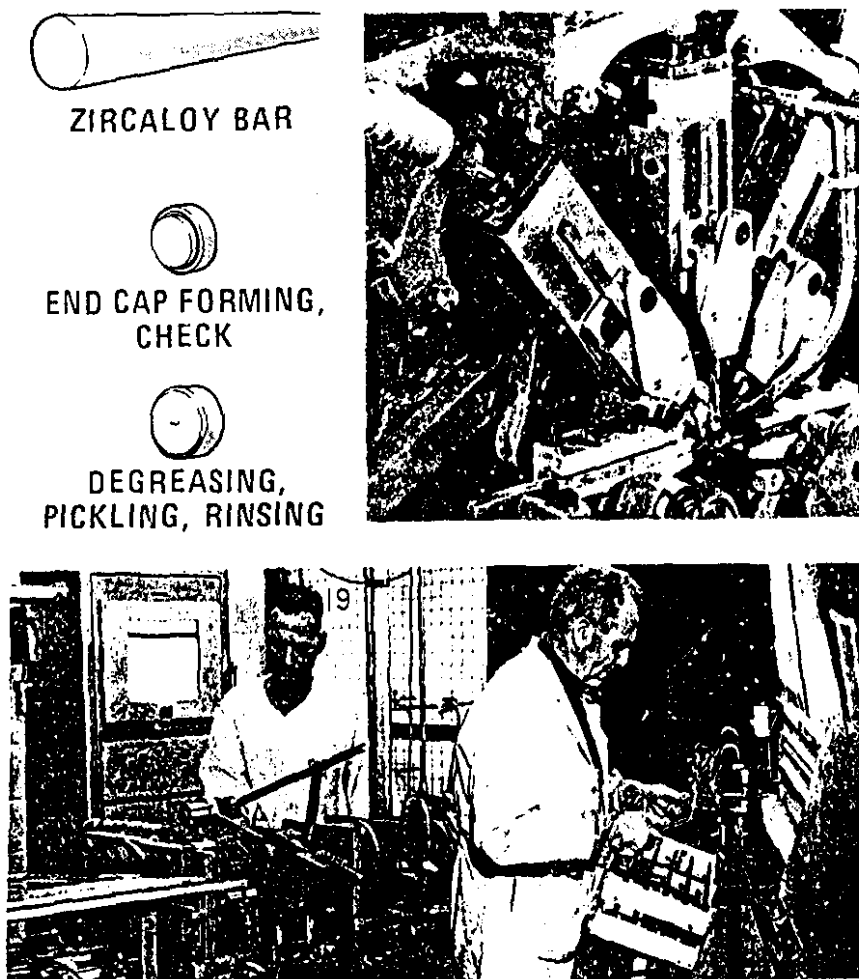
FIGURE 17 Fuel Bundle Production Stage 2
