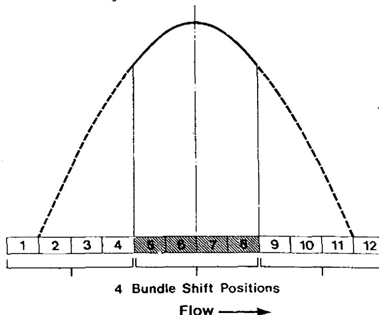
FIGURE 41 Douglas Point Axial Flux Profile
