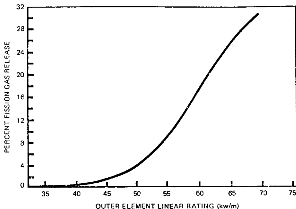
FIGURE 20 Percent Fission Gas Release versus \text{UO}_2 Power Rating
