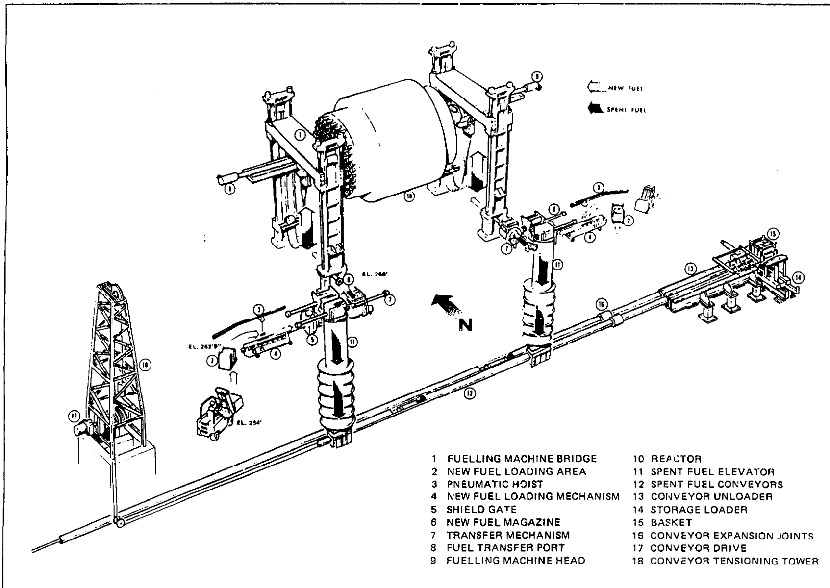
FIGURE 28 Pickering Fuel Handling System
