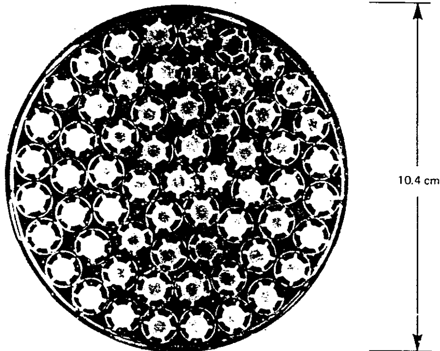
FIGURE 44 Gentilly Booster Cross Section
