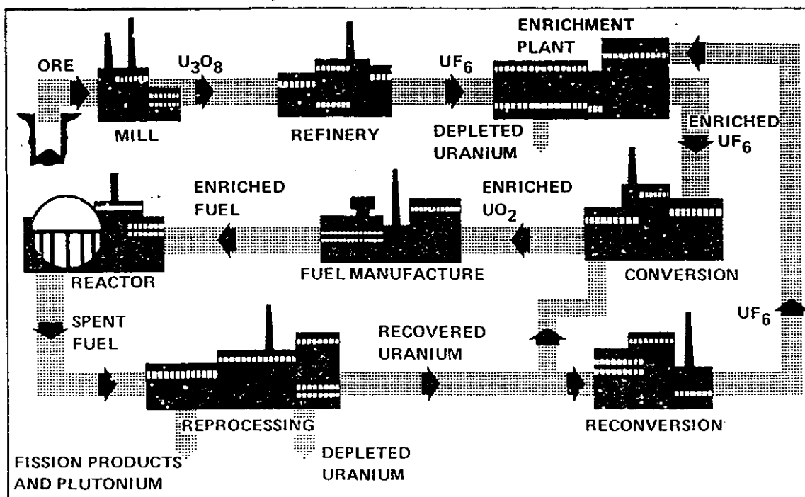
FIGURE 6 Enriched Uranium Cycle
