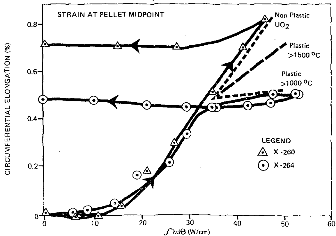
FIGURE 26b Mid Plane Circumferential Strains, ditto
