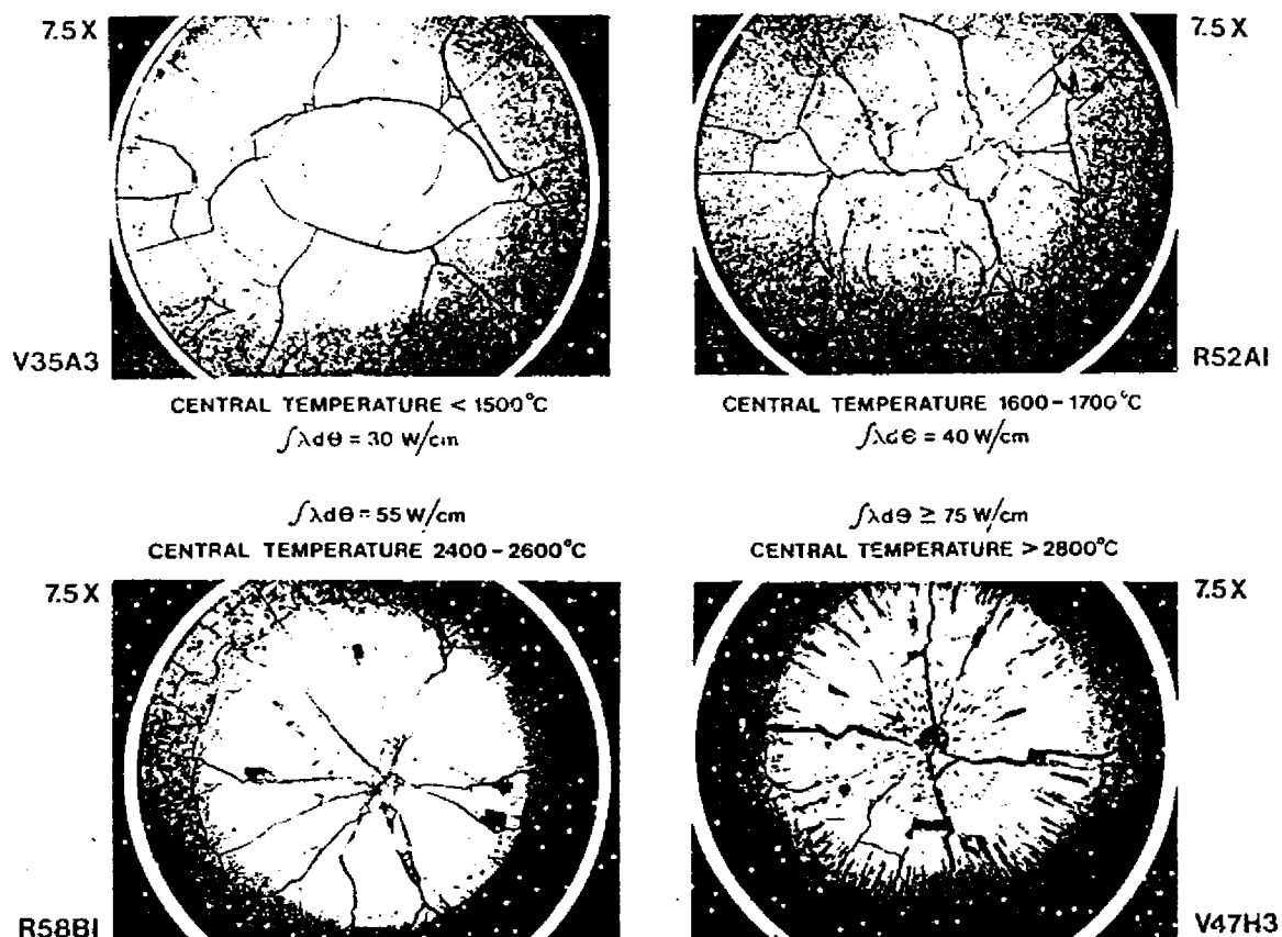
FIGURE 19 Typical Transverse Cross Section of Irradiated \text{UO}_2 at Four Power Ratings showing Pellet Cracks and \text{UO}_2 Grain Growth
