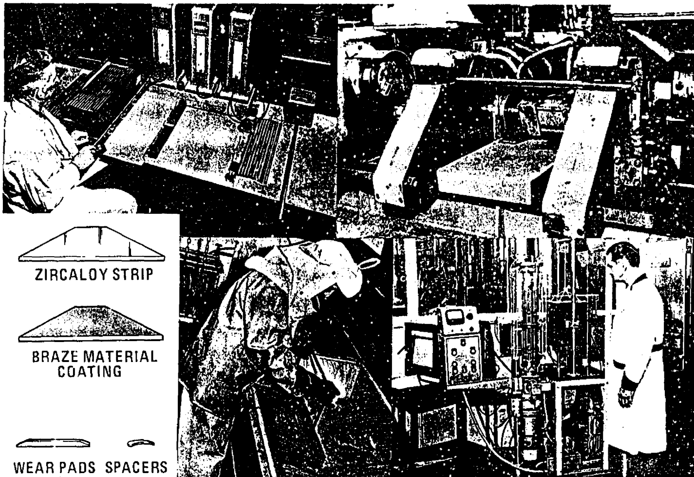
FIGURE 16 Fuel Bundle Production Stage 1
